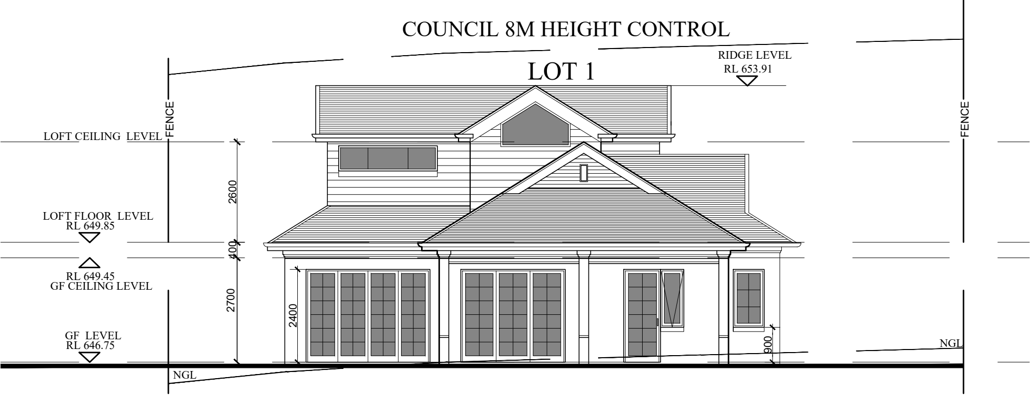
NORTHEAST ELEVATION - LOT 1 SCALE - 1:100
