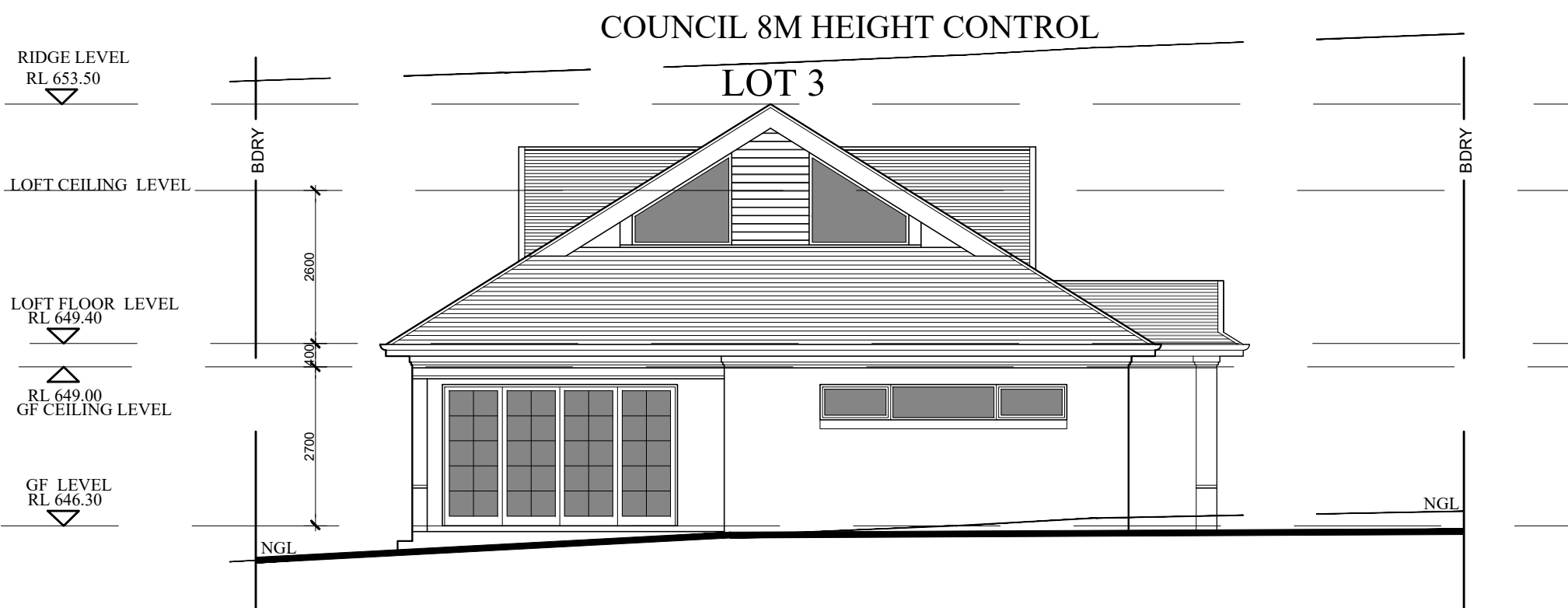
NORTHEAST ELEVATION - LOT 3 SCALE - 1:100
