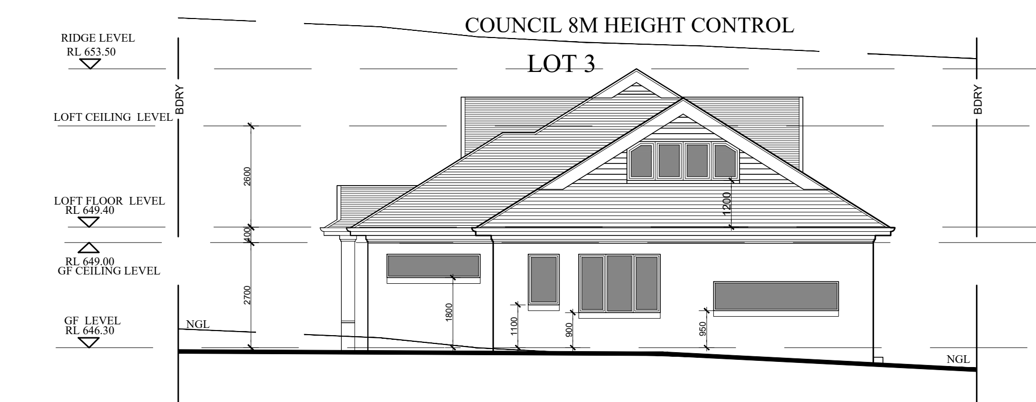
SOUTHWEST ELEVATION - LOT 3 SCALE - 1:100
