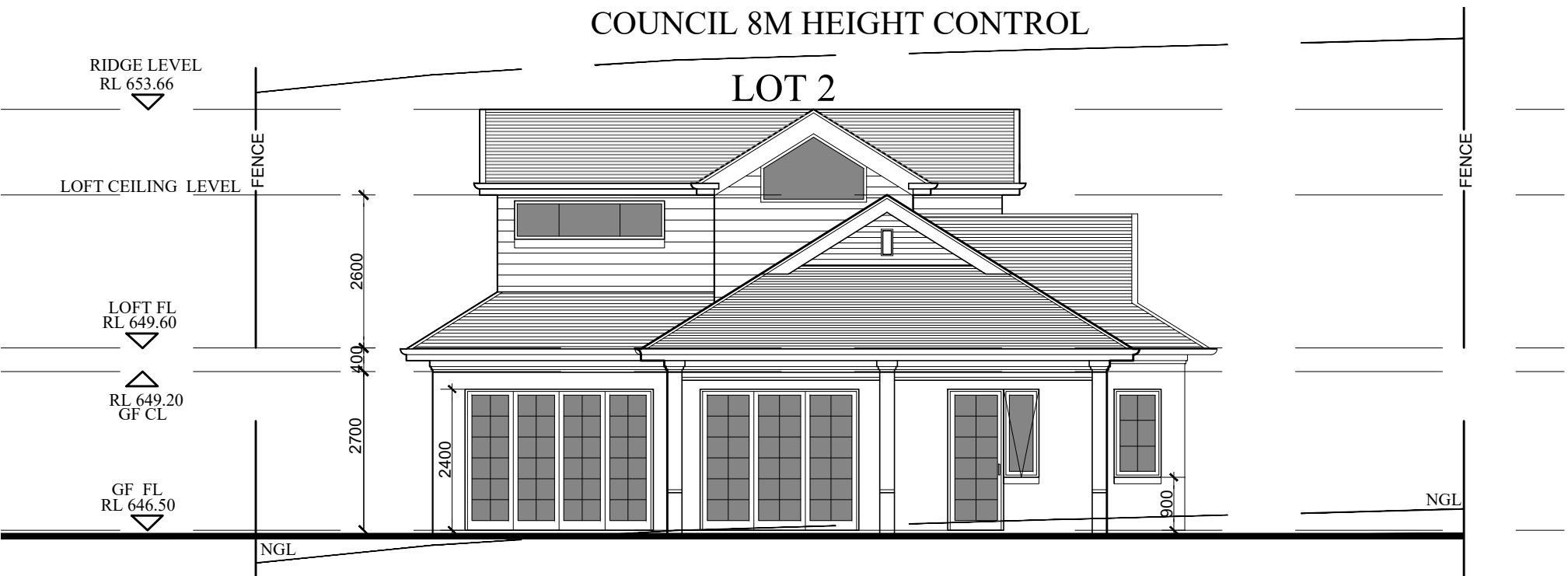
NORTHEAST ELEVATION - LOT 2 SCALE - 1:100
