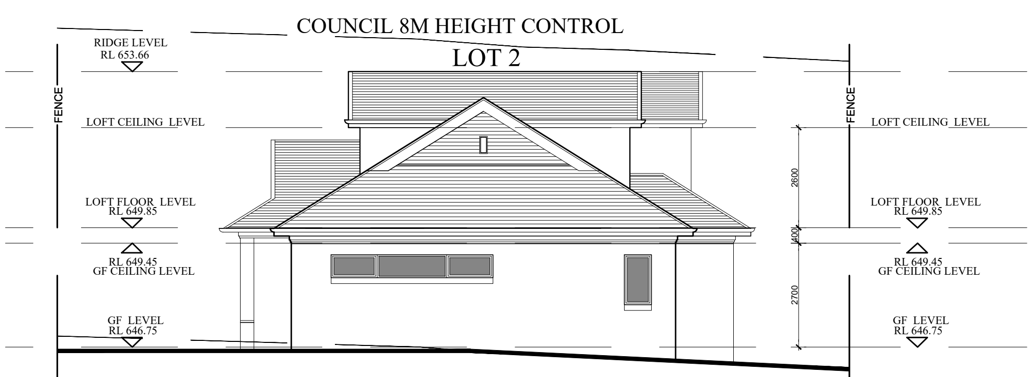
SOUTHWEST ELEVATION - LOT 2 SCALE - 1:100
